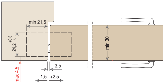
Door cross-section
