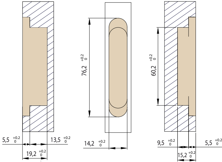
Slot measurement
