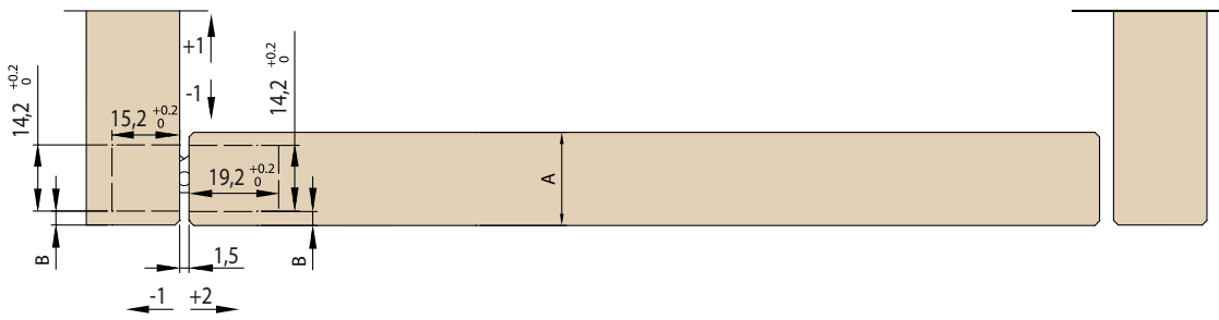
Cabinet cross-section with door inside the box
