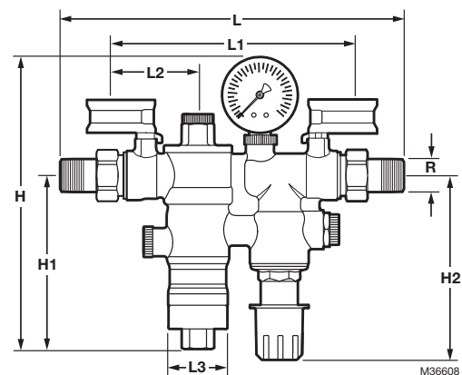
Fig. 1. Dimensions.
